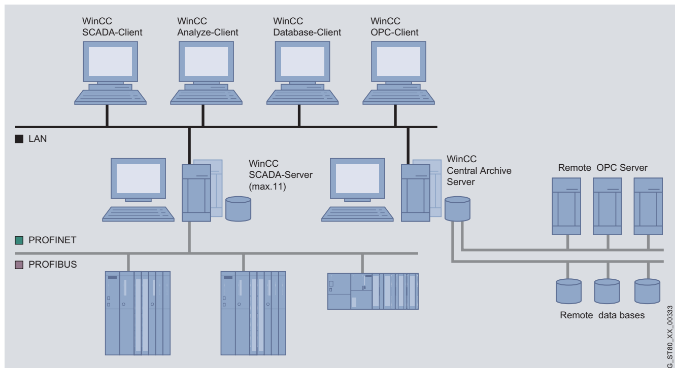
Central process data archiving
