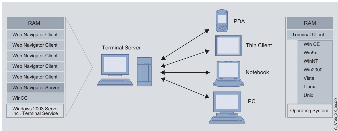
Thin clients on various operating system platforms on the WinCC/WebNavigator server
