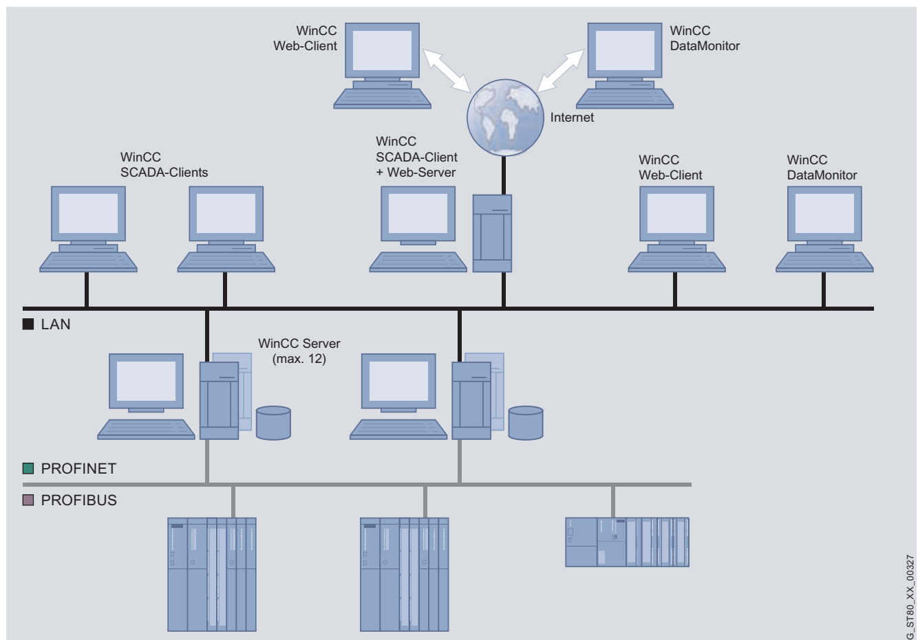
WinCC SCADA Clients as web server for different clients in the web
