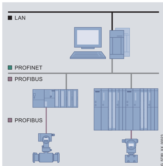
WinCC single-user system
