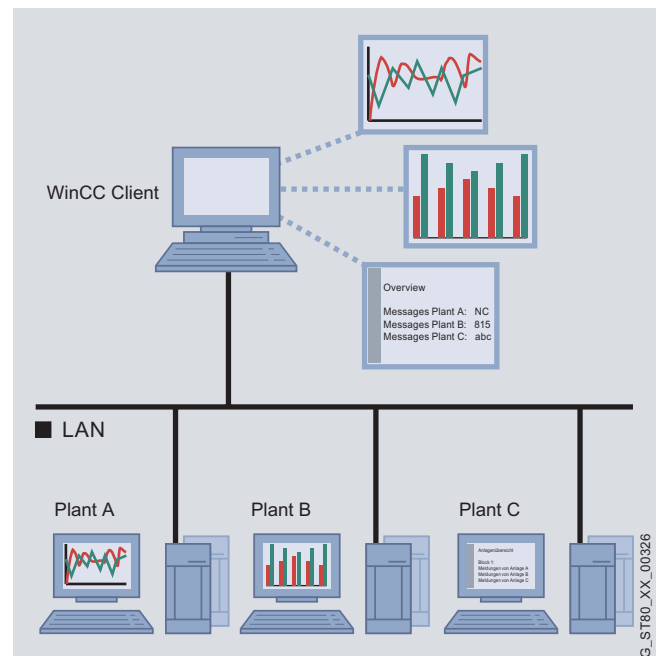
Distribution of the servers according to plant sections
