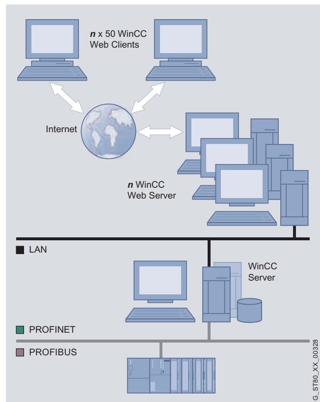
Web server farms (Load Balancing) with many web clients
