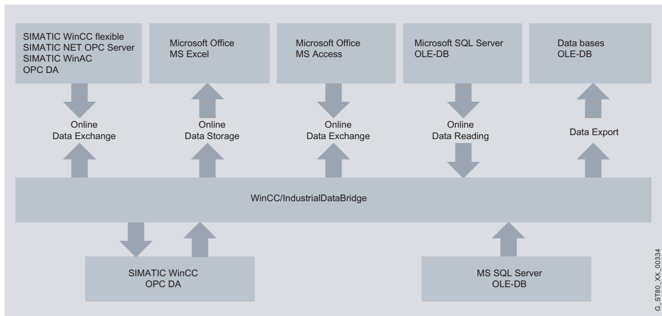
WinCC/IndustrialDataBridge: Connection to databases and IT systems
