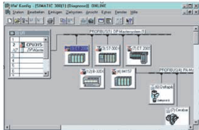
Call-up of the STEP 7 hardware diagnostics from WinCC
